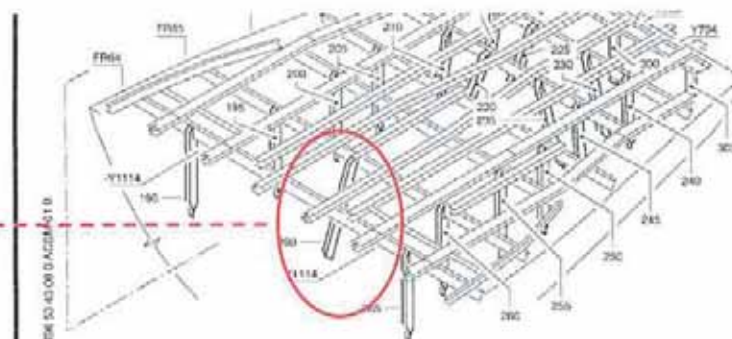
FR60-FR70 - Support Struts Figure 1 (sheet 2)
